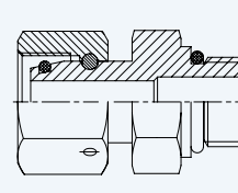
DIN 2353 Swivel Female Connector SAE MALE with O Ring
