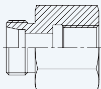
Female Connector BSPP Female
