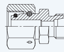
Swivel Reducing Connector with 24° Cone L Series
