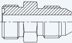
Straight Connector ORFS Male - JIS BSPP Male 60° Cone
