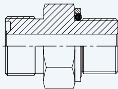
Straight ORFS Male - BSPP Male + Retaining Ring + O Ring
