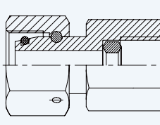
Swivel Connector (Metric Female) with 24° Cone and DKl
