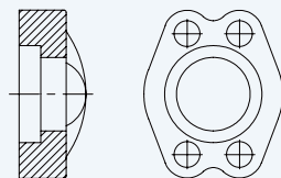
Captive Flange SAE Code 61
