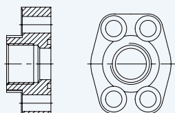
4 Bolt Thread Flange, BSPP Female Code 61
