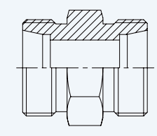
Straight Connector
