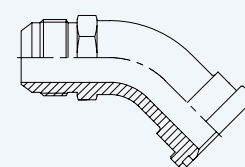
45° Swept Elbows JIC Male 74° - Flange SAE Code 61
