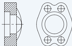
Captive Flange SAE Code 62
