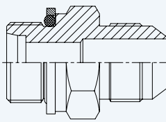
DIN 2353 Male Connector O Ring and Retaining Ring (JIC male)
