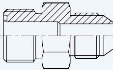
Straight Connector ORFS Male - JIC 74° Male
