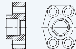
4 Bolt Thread Flange, BSPP Female Code 62
