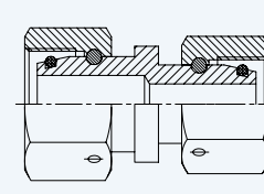
DIN 2353 Swivel Female Reducing Coupling with 24° Cone
