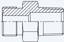
Straight Connector ORFS Male - BSPT 60° Male
