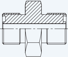
Straight Connector ORFS Male - ORFS Male
