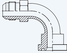
90° Swept Elbows JIC Male 74° - Flange SAE Code 62
