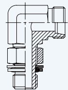
Adjustable Elbow Metric Male ORB
