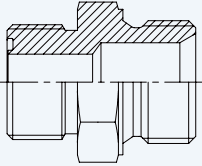
Straight Connector ORFS Male - Metric 60° Male Cone
