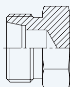
Tube Cap
