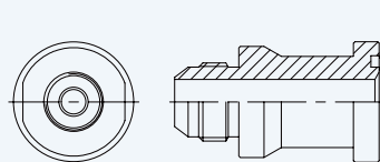
Straight Connector JIC Male - Flange SAE Code 62
