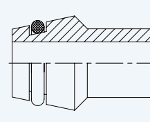
Welding Nipple with O Ring
