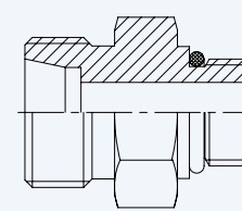
Male Connector (JIC Male) with O Ring
