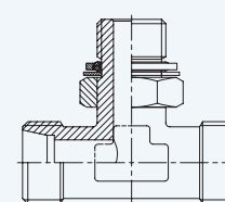
DIN 2353 Adjustable Branch Tee with BSPP Male + O Ring + Retaining Ring
