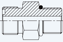
Straight Connector ORFS Male - SAE Male + O Ring
