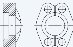
Split Flange SAE Code 62
