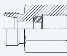
Female Connector Metric Female With DKl
