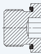
Blanking Plug Metric for Port with ED Ring
