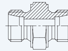
Reducing Straight Connector Large Hexagon
