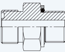
Straight ORFS Male - Metric Male + Retaining Ring + O Ring
