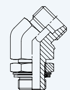
DIN 2353 Adjustable Elbow 45° Metric Male O Ring and Retaining Ring
