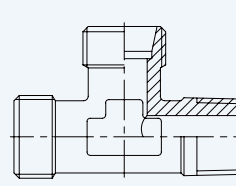
Adjustable Run Tee with BSPT Male
