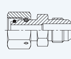
Swivel Female Connector JIC Male with 24° Cone
