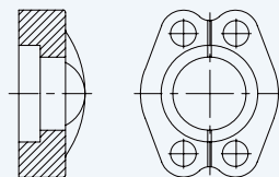
Split Flange SAE Code 61
