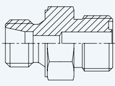
DIN2353 Male Connector ORFS Male
