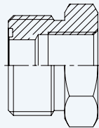
Straight Connector ORFS Male - BSPP Fixed Female
