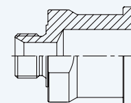
Straight Connector BSPP Male 60° - Flange SAE Code 61
