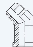
45° Forged Elbows JIC Male 74° - Flange SAE Code 61
