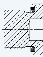
Blanking Plug BSPP for Port with ED Ring
