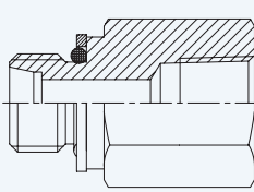
Male Connector (NPTF Male) with Form X Tapped Holes
