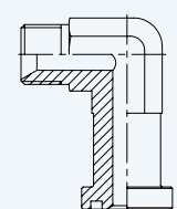
90° Forged Elbows BSPP Male 60° - Flange SAE Code 62
