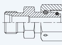
Swivel Female Connector with 24° Cone
