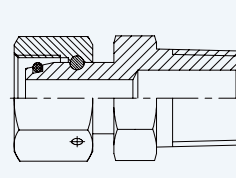
Swivel Female Connector (NPTF Male) with 24° Cone
