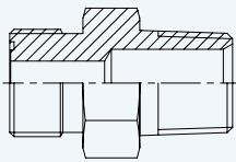
Straight Connector ORFS Male - NPTF 60° Male
