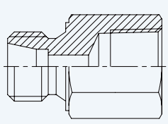
Female Connector NPTF Female
