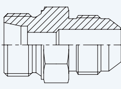
Male Connector (JIC male)
