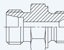
Male Connector (BSPP Male) with 60° Cone Seal
