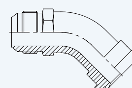
45° Swept Elbow JIC Male 74° - Flange SAE Code 62
