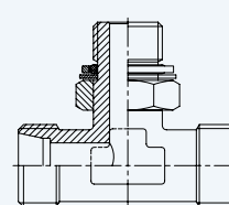
DIN 2353 Adjustable Branch Tee with Metric Male O Ring and Retaining Ring
