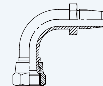
90° Swept Elbows JIC Swivel Female - Reusable Tail for R1/R2/R5
