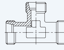
Reducing Tee
