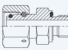
Swivel Female Connector (BSPP Male) with 24° Cone and ED Ring
