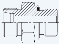
Male Connector (BSPP Male) with ED Ring
