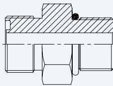
Straight Connector ORFS Male - BSPP Male + O Ring
