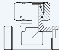
Swivel Adjustable Branch Tee with 24° Cone
