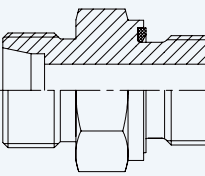
Metric Male Connector with ED Ring
