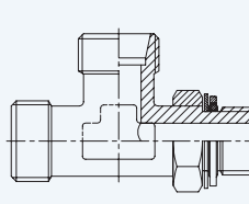
DIN 2353 Adjustable Run Tee with BSPP Male + O Ring + Retaining Ring
