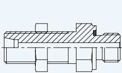
Male Bulkhead Connector (BSPP) with ED Ring
