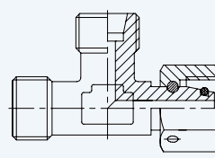
Swivel Adjustable Run Tee with 24° Cone
