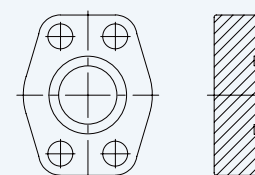
Blind Flanges Low Pressure SAE Code 61
