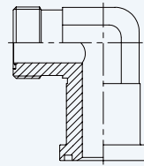
90° Forged Elbow ORFS Male - Flange SAE Code 62
