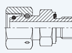
Swivel Female Connector (Metric Male) with 24° Cone and ED Ring
