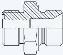
Straight Connector ORFS Male - BSPP 60° Male
