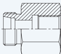
Female Connector Metric Female
