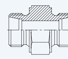
Straight Connector Large Hexagon
