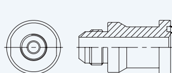
Straight JIC Male 74° - Flange SAE Code 61
