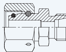
Swivel Reducing Connector with 24° Cone S Series
