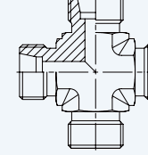
Connector Cross
