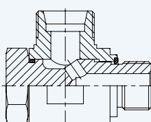
Banjo Coupling BSPP with ED Ring
