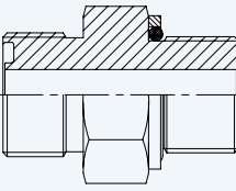
Straight Connector ORFS Male - Metric Male + O Ring
