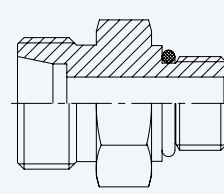
DIN2353 Male Connector Metric Male with O Ring
