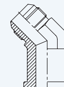
45° Forged Elbow JIC Male 74° - Flange SAE Code 62
