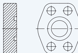
Blind Flanges Zero Pressure SAE Code 61
