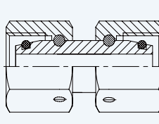
Swivel Female Connector with 24° Cone
