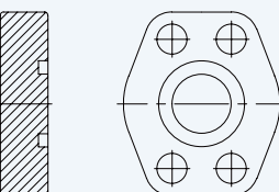
Blind Flanges Zero Pressure SAE Code 62
