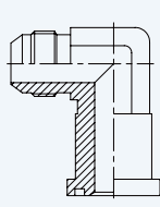
90° Forged Elbow JIC Male 74° - Flange SAE Code 61
