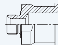
Straight Connector BSPP Male 60° - Flange SAE Code 62
