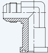
90° Forged Elbow JIC Male 74° - Flange SAE Code 62
